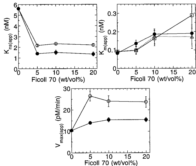
FIGURE 5 Comparison of calculated ( \circ , \square , \triangle ) and measured ( \bullet ) apparent kinetic parameters in Ficoll 70 solutions. K_{d,ns(app)} and V_{max(app)} calculations are based on excluded volume effects and include compensation for changes in water activity. The K_{m(app)} calculation also accounts for changes in diffusion by use of a stretched exponential equation ( \square ) or the Einstein relation ( \triangle ) as described in the text.
